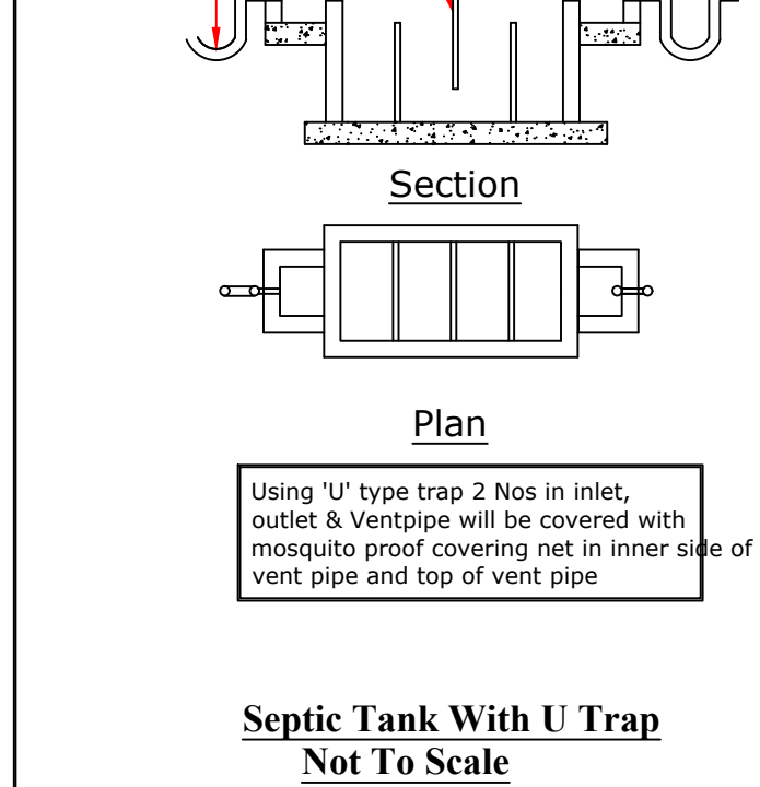
LAYOUT BY:-
