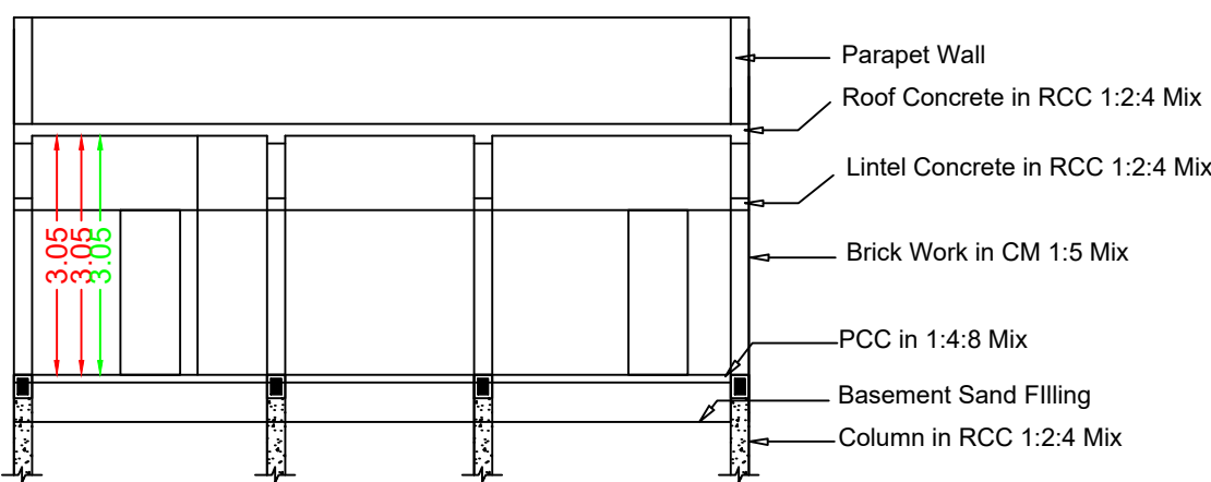
Section RR
