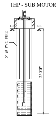
BOREWELL DETAILS
