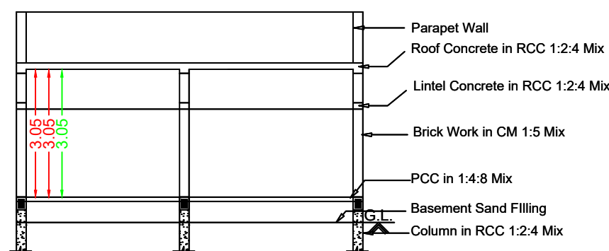
Section RR
