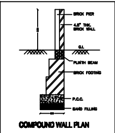
COMPOUND WALL PLAN
