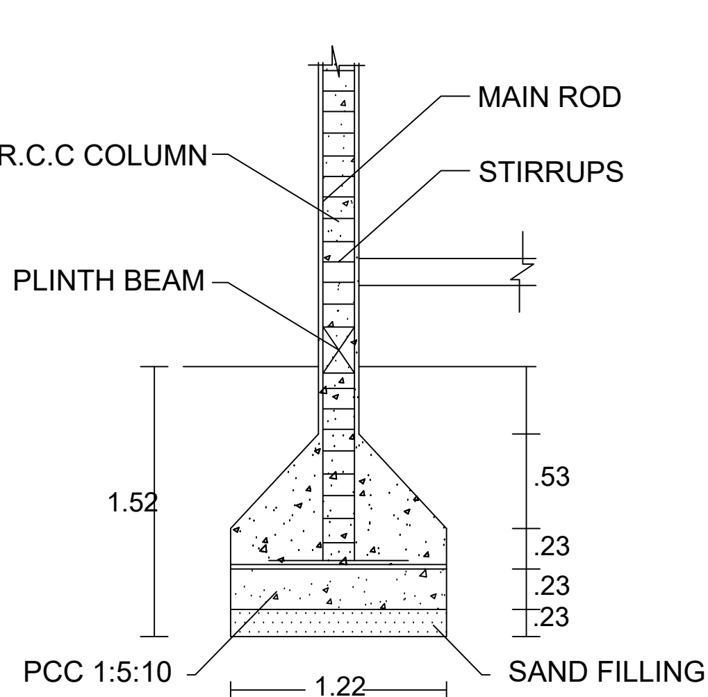
COLUMN DETAILS
