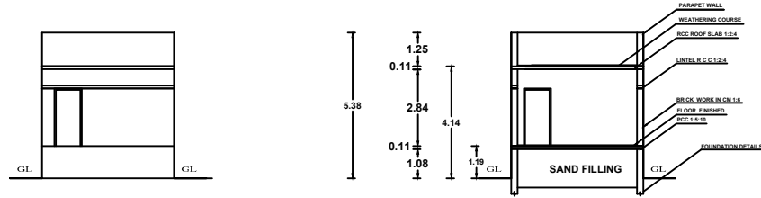
FRONT ELEVATION
