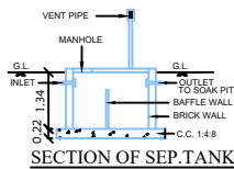
SECTION OF SEP.TANK
