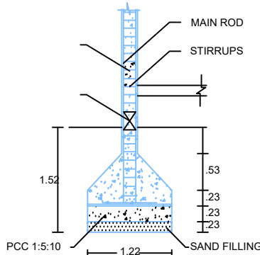
COLUMN DETAILS
