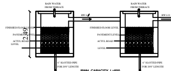
RAIN WATER STORAGE TANKS
