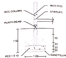
COLUMN DETAILS
