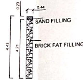
DETAILS OF PERCOLATION PIT
