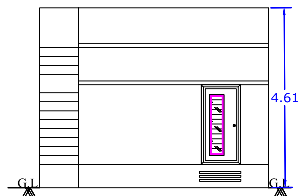
FRONT ELEVATION
