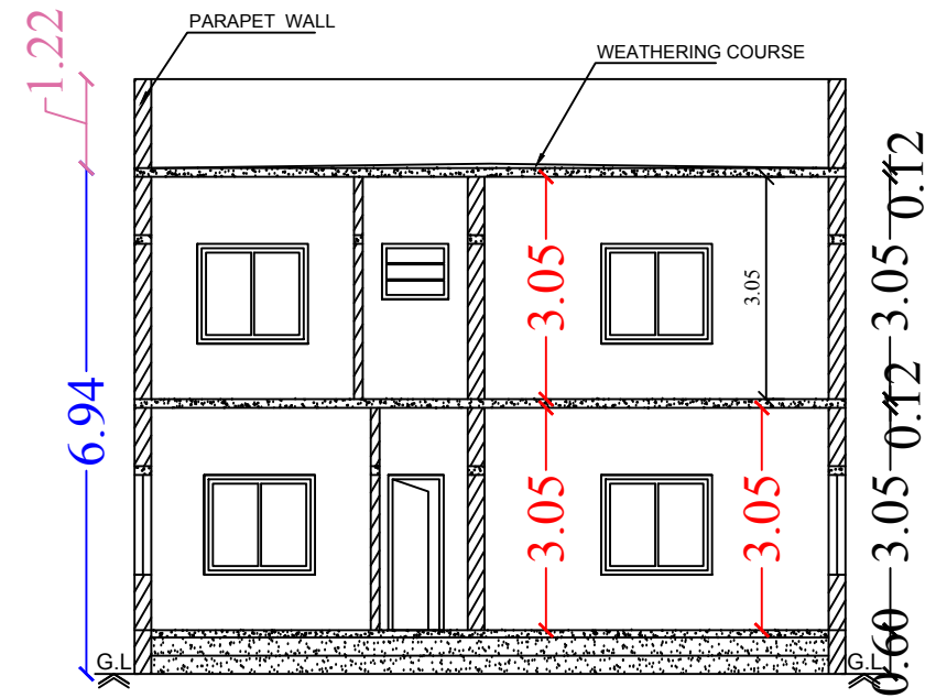
Section on-"AA"
