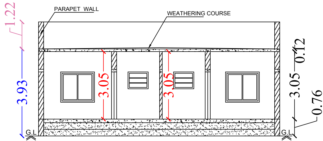
Section on-"AA"
