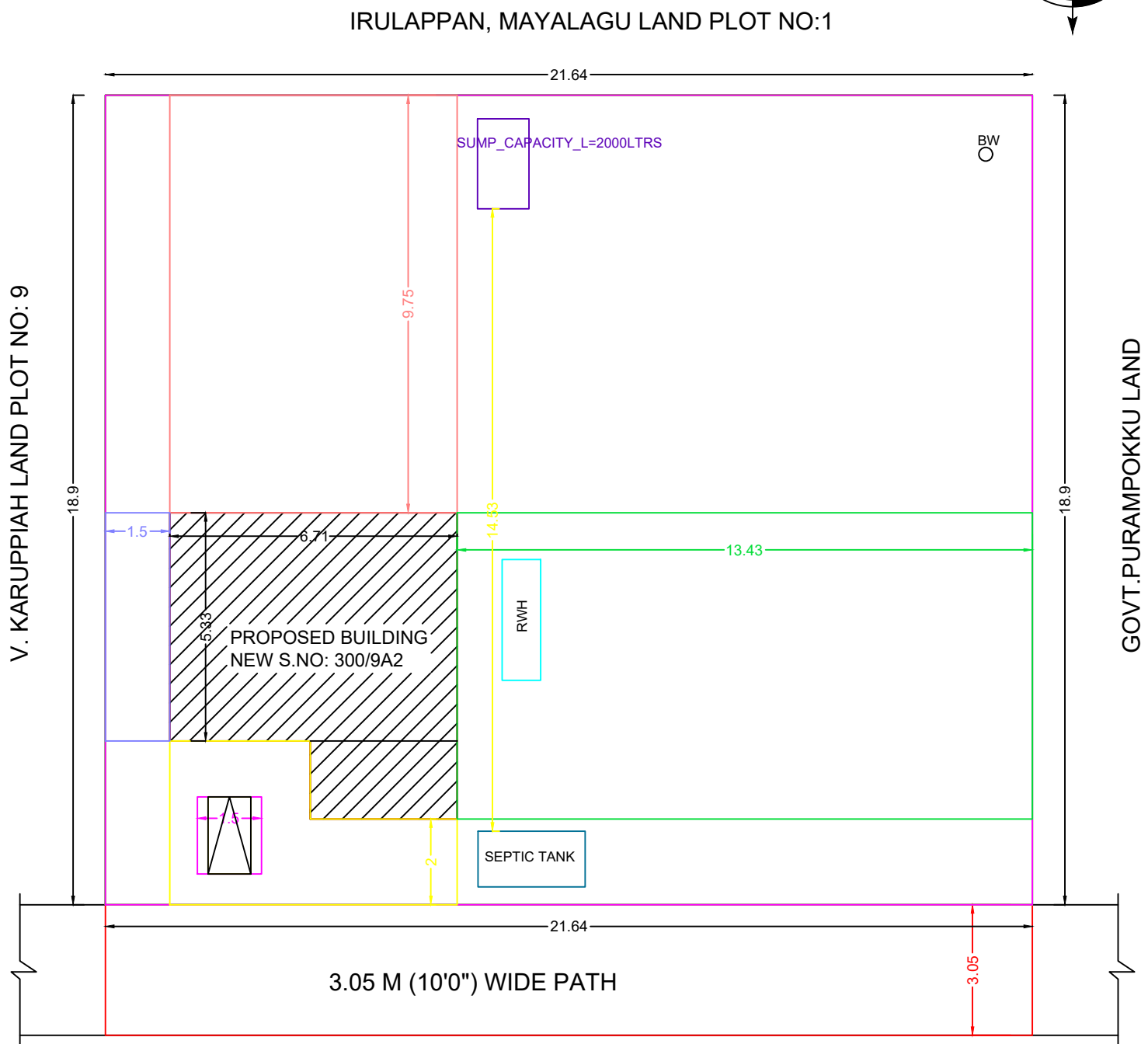
SITE PLAN
