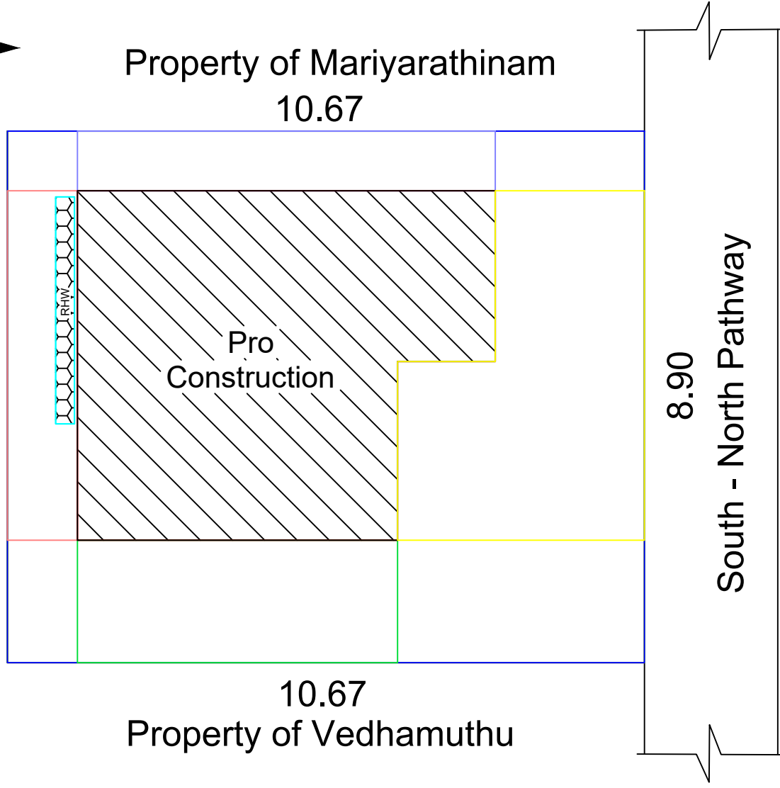
Site Plan
