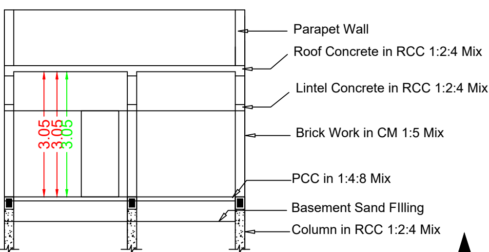
Section RR
