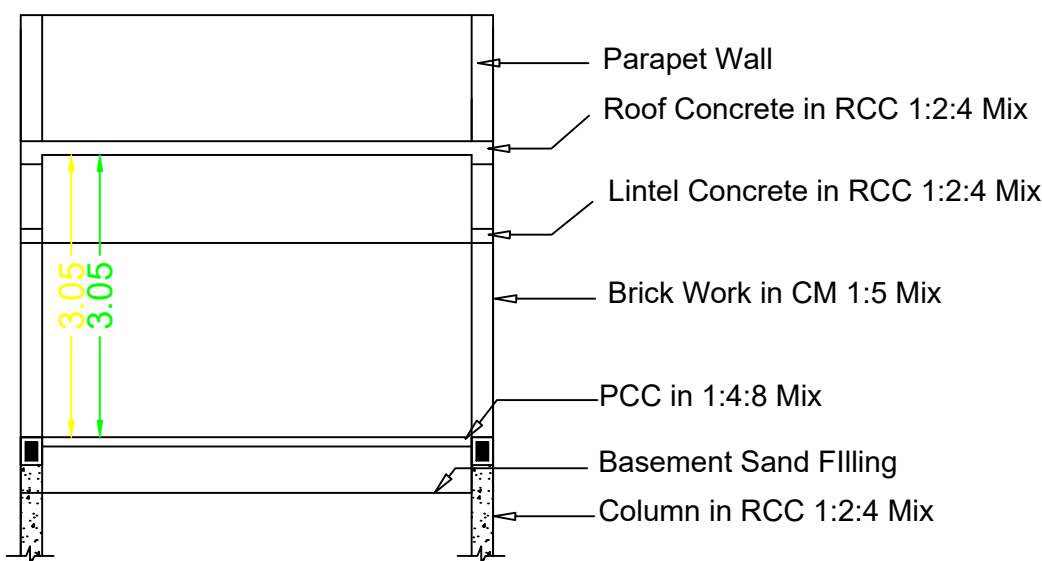
Section RR
