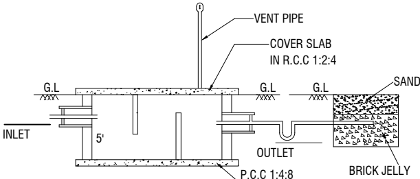
SECTION-AB
