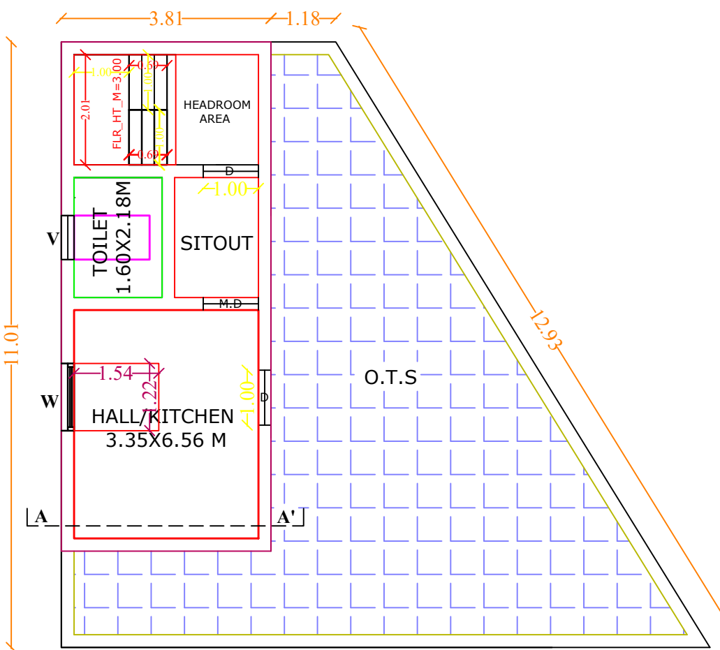
PRO SECOND FLOOR PLAN
