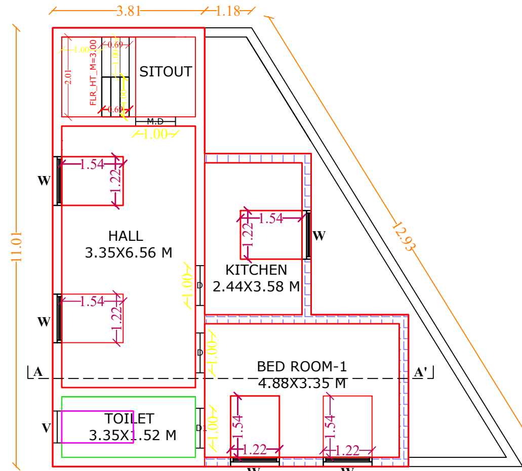
EXT AND EXTN FIRST FLOOR PLAN
