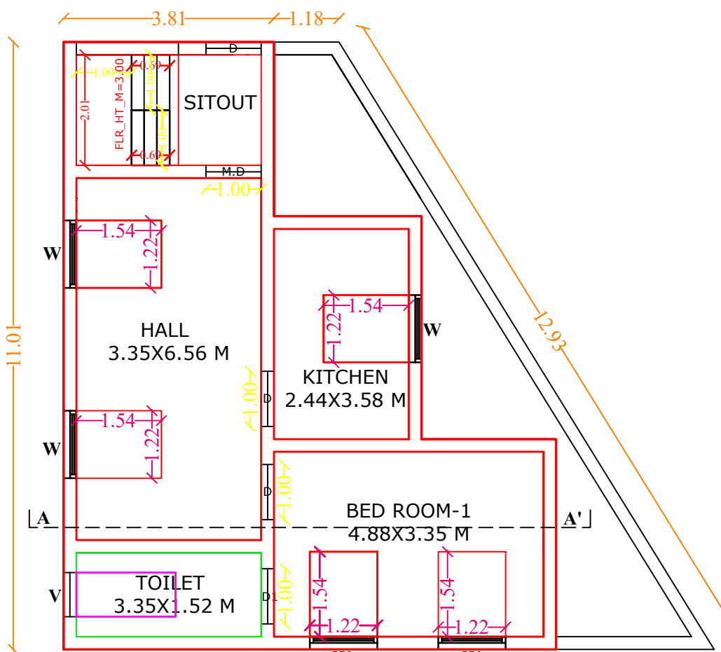
EXT GROUND FLOOR PLAN
