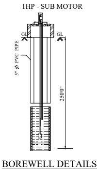
BOREWELL DETAILS
