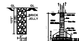
PERCULATION PIT
