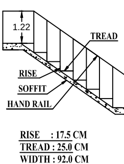
STAIRCASE DETAILS (NTS)
