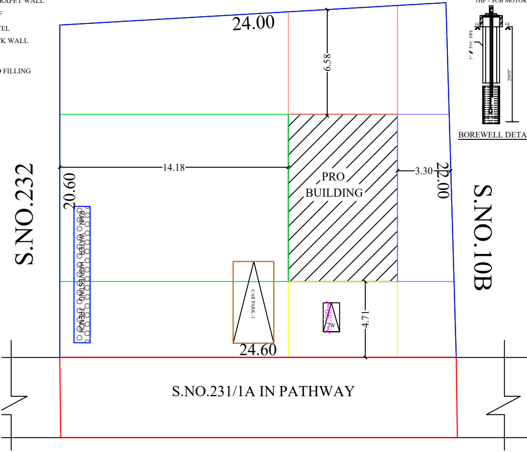
SITE PLAN
