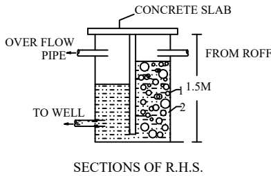
SECTIONS OF R.H.S.
