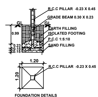
FOUNDATION DETAILS
