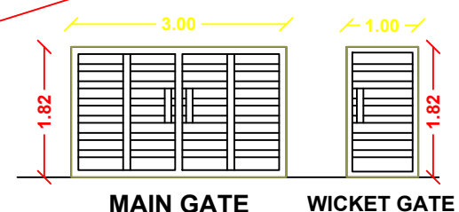
MAIN GATE WICKET GATE
