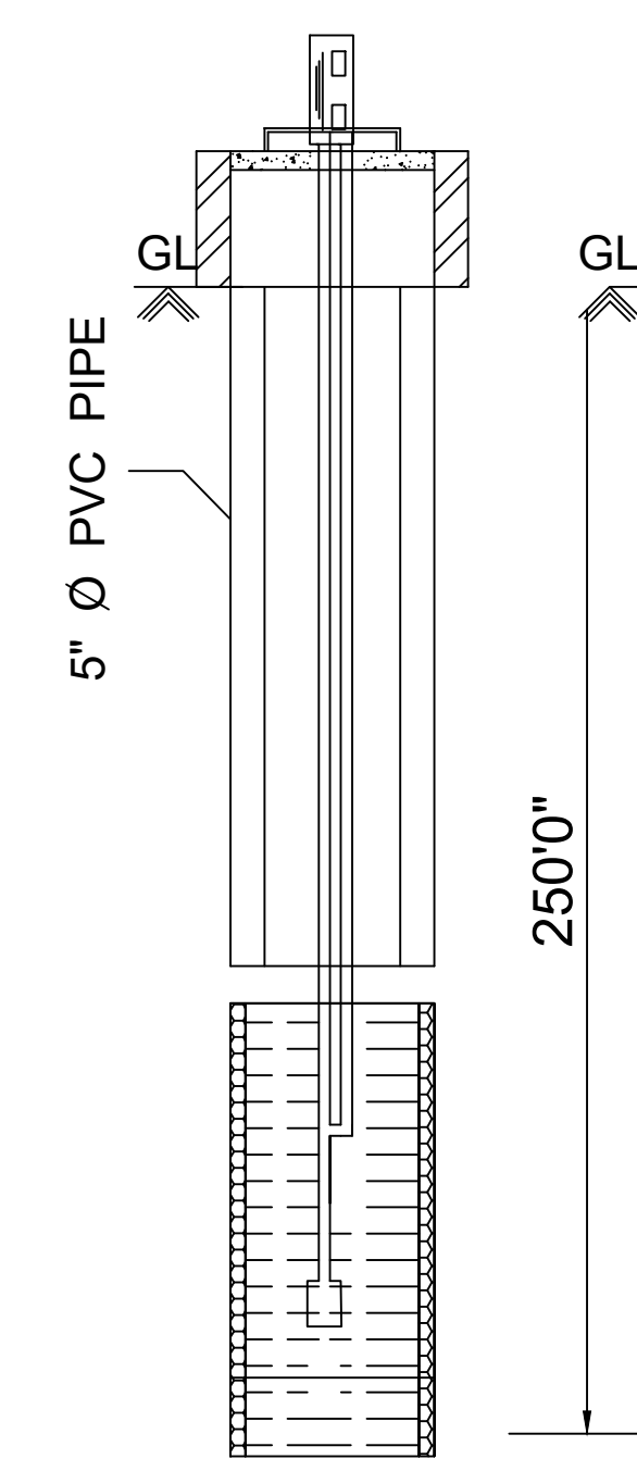
BOREWELL DETAILS
