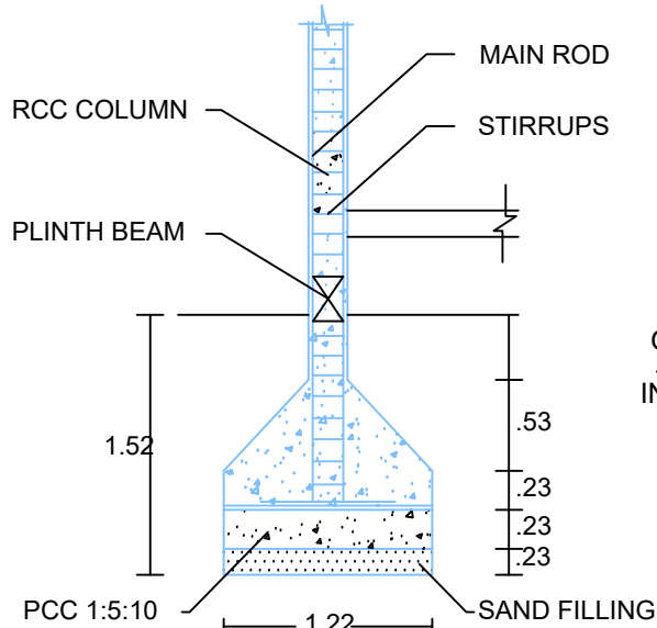
COLUMN DETAILS
