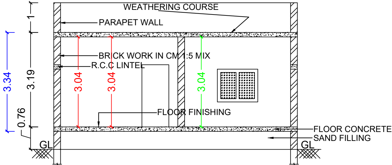
SECTION AT A1-A1
