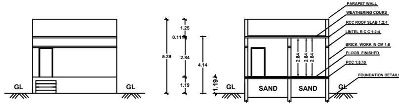
SECTION ON "A B"
