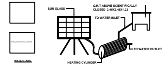
SOLAR WATER HEATING SYSTEM
