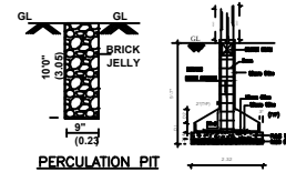
PERCOLATION PIT
