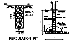
PERCOLATION PIT FOUNDATION DETAILS SCALE : 1:50.
