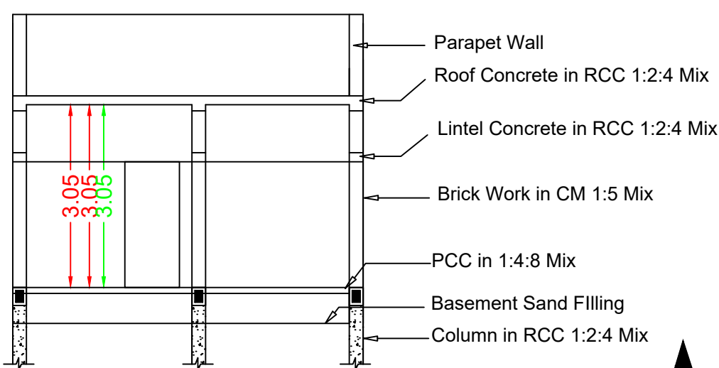
Section RR
