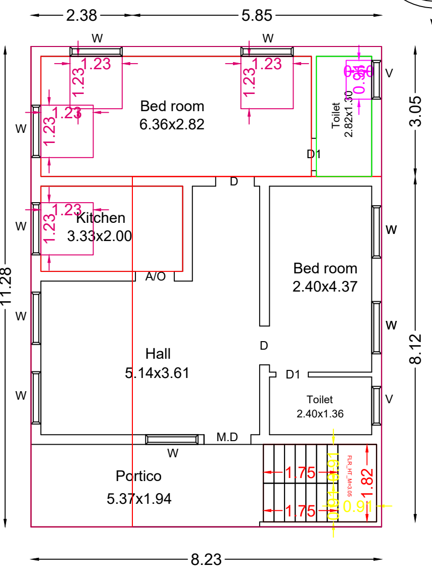
Ex & Pro.Ground Floor Plan
