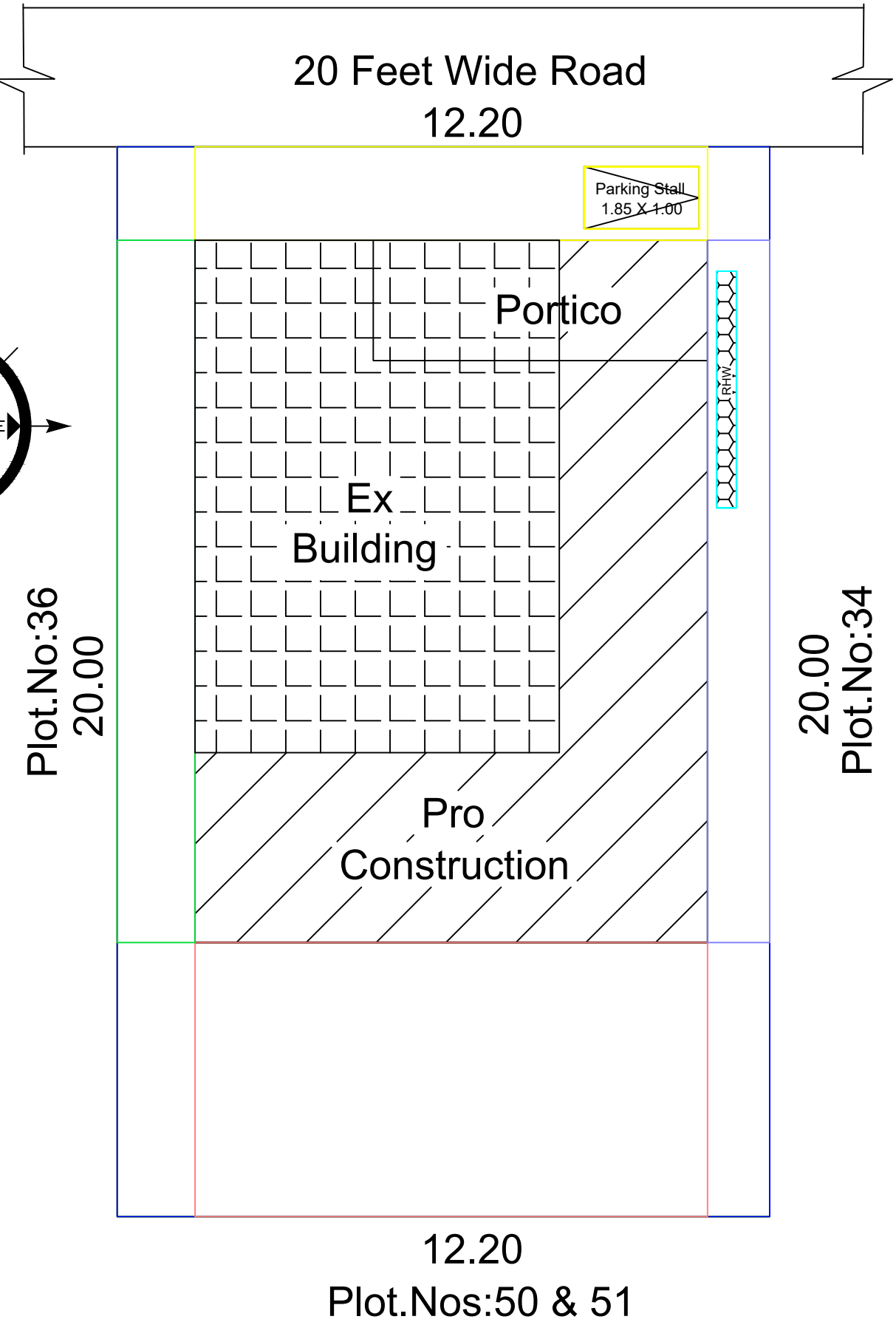
Site Plan(NTS)
