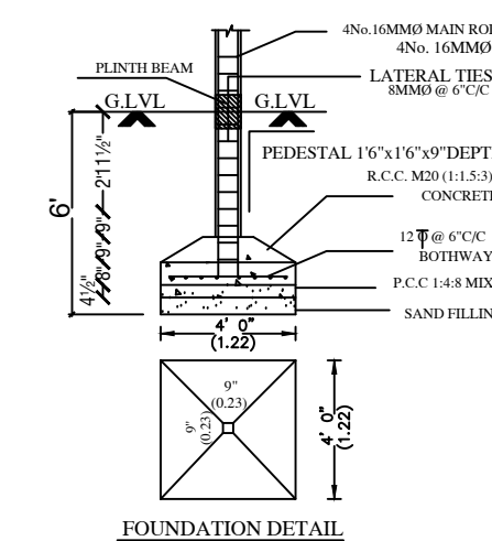
FOUNDATION DETAIL
