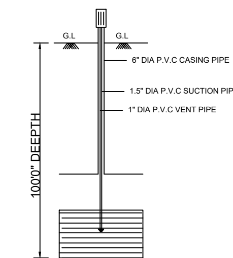
BORE WELL
