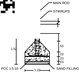
COLUMN DETAILS
