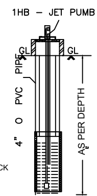
SECTION OF BORE WELL
