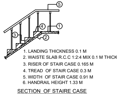
SECTION OF STAIRE CASE
