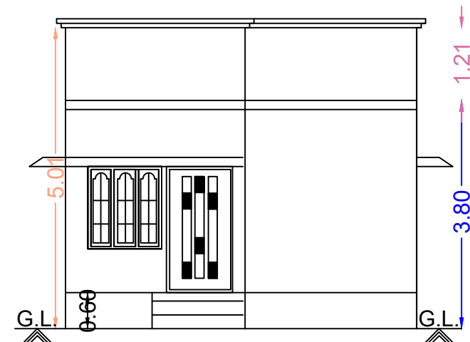
Front Elevation
