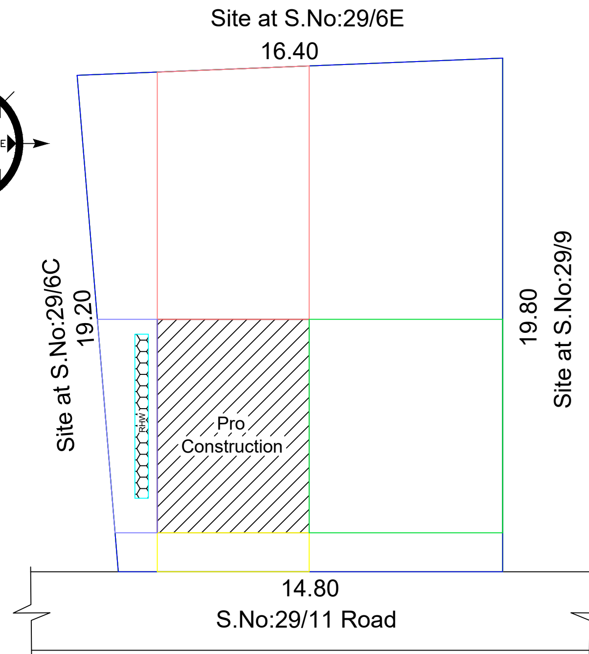
Site Plan(NTS)
