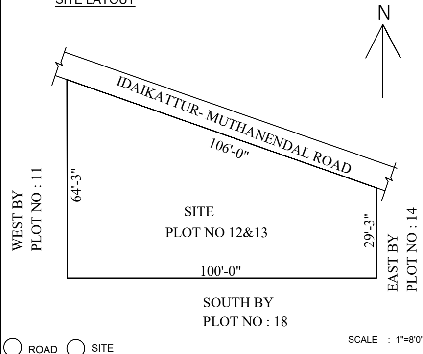
SITE LAYOUT
