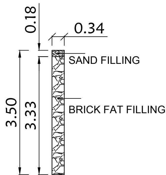
DETAILS OF PERCULATION PIT
