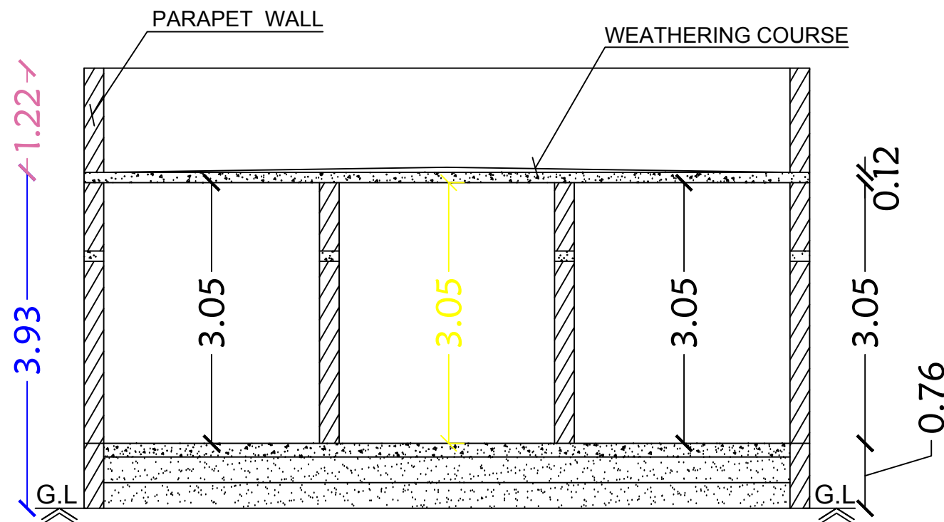
Section on-"AA"
