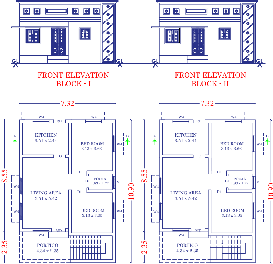
GROUND FLOOR PLAN BLOCK - I
