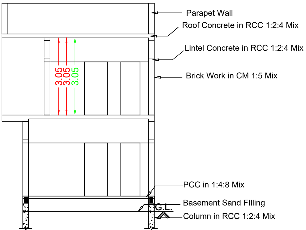
Section RR
