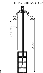
BOREWELL DETAILS
