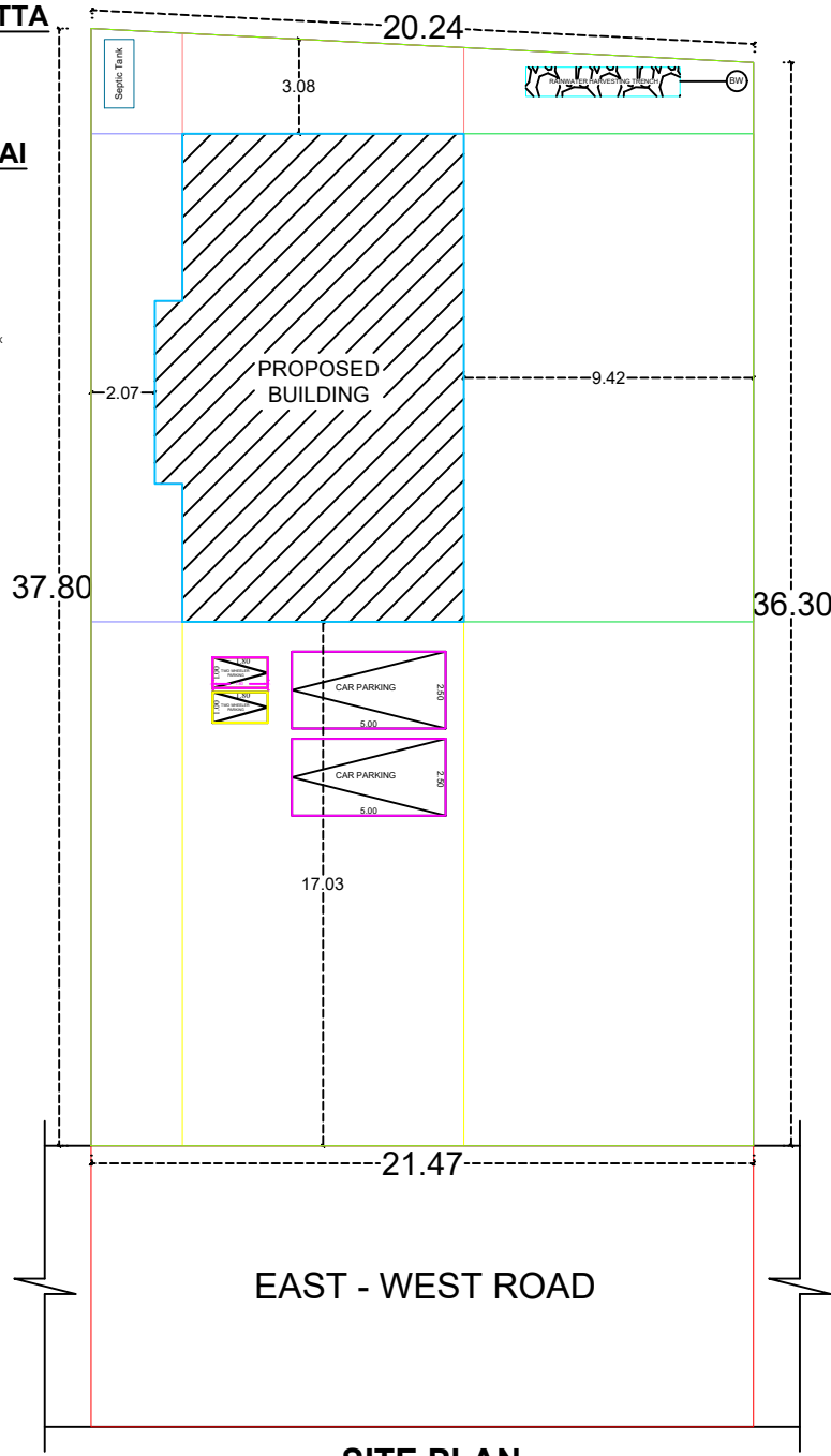
SITE PLAN (1:100)
