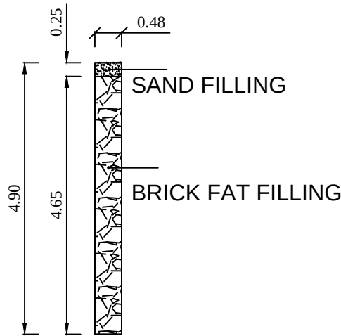
DETAILS OF PERCULATION PIT
