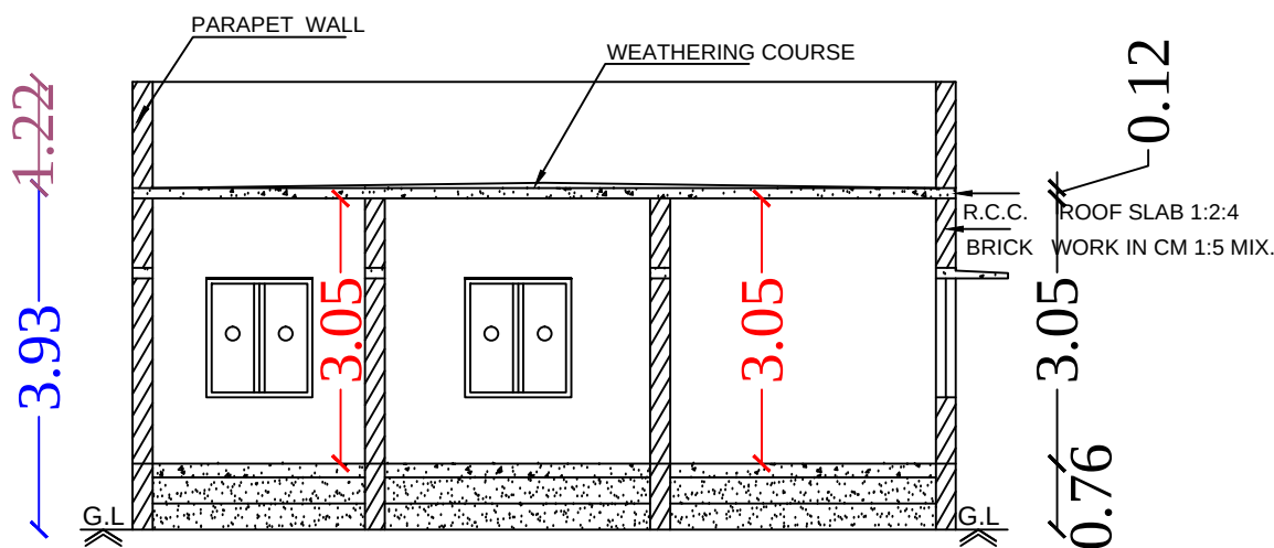
Section on-"AA"
