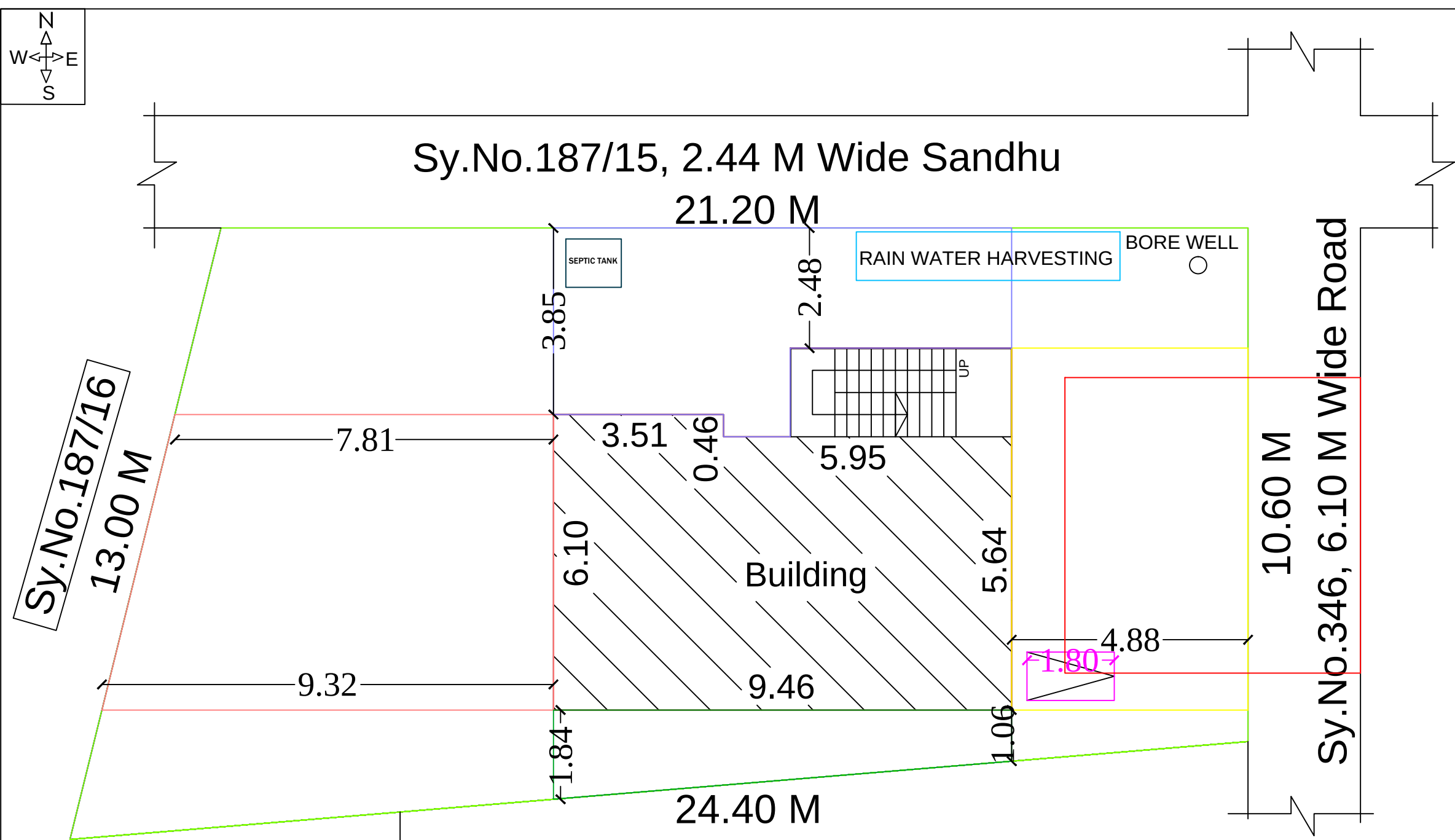
SITE PLAN
