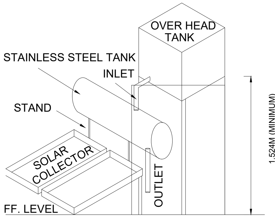
SOLAR WATER HEATING SYSTEM
