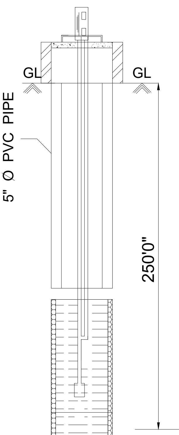
BOREWELL DETAILS
