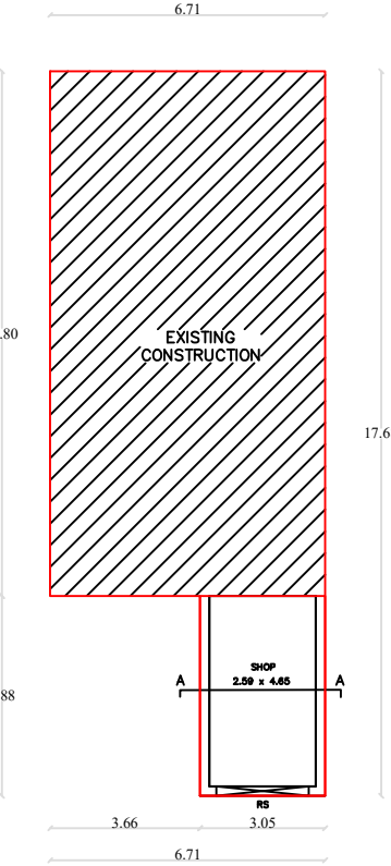
PRO.GROUND FLOOR PLAN
