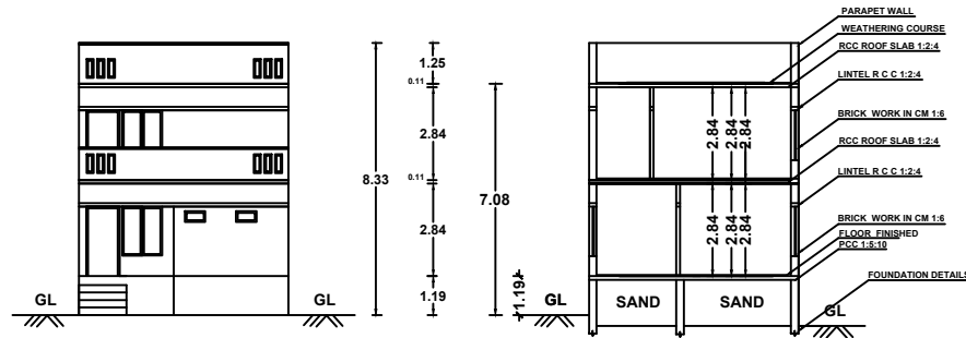
FRONT ELEVATION
