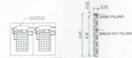
DETAILS OF PERCUSSION PIT
