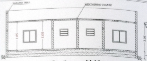
Section on-"AA"
