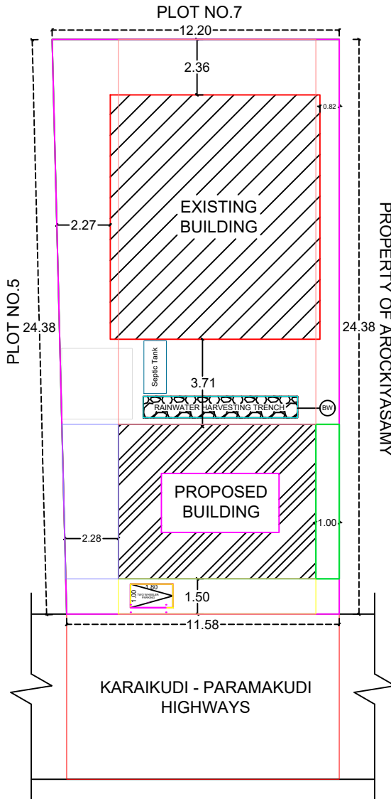
SITE PLAN (1:100)
