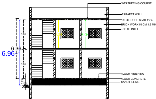
SECTION A1-A1
