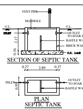
SECTION OF SEPTIC TANK
