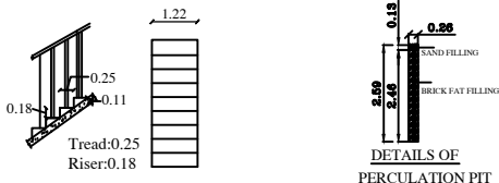
STAIRCASE DETAIL
