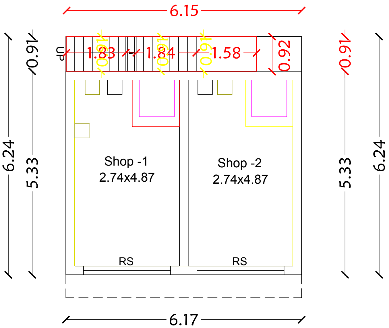
Ground Floor
