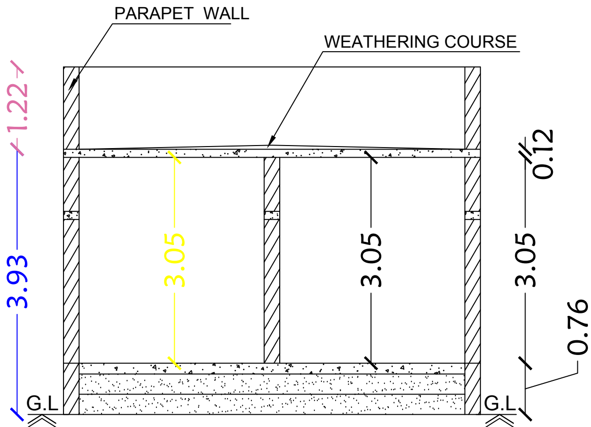
Section on-"AA"
