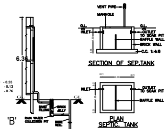
PLAN SEPTIC TANK
