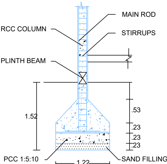
COLUMN DETAILS
