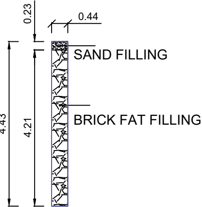
DETAILS OF PERCULATION PIT
