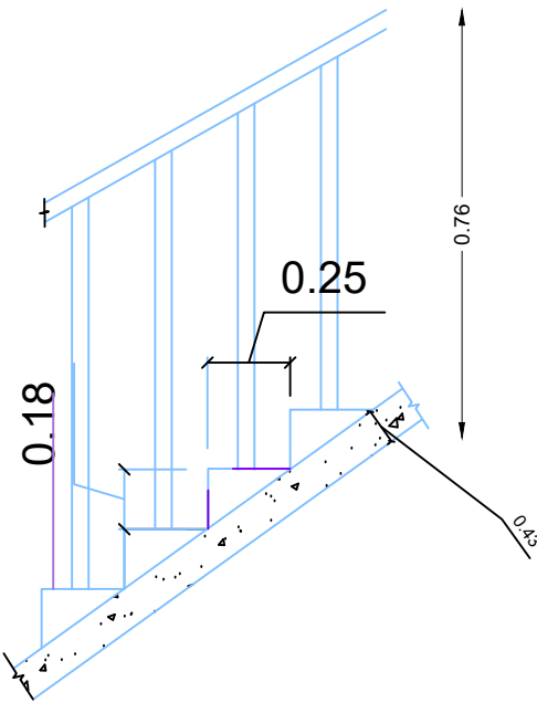
SECTION OF STAIRCASE
