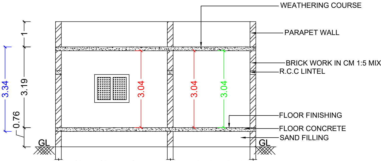
SECTION AT A1-A1
